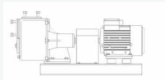
VAC 2000 with free shaft end. VAC 2000 is complete with flexible coupling and electric motor 2.2 kW at 2850 RPM.
